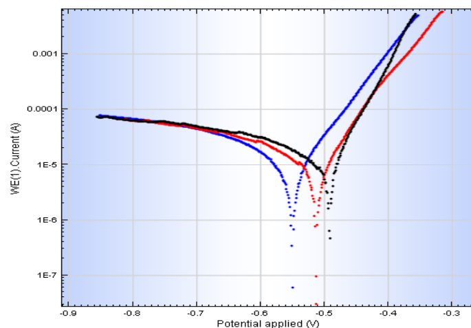
Figure 3. Polarization Curves Recorded in 1 M Na 2 CO 3 Solution at 10 mv/s for the bulk of CHT and DCT Samples. (Note: ■ CHT, ■ DCT, ■ SCT)
