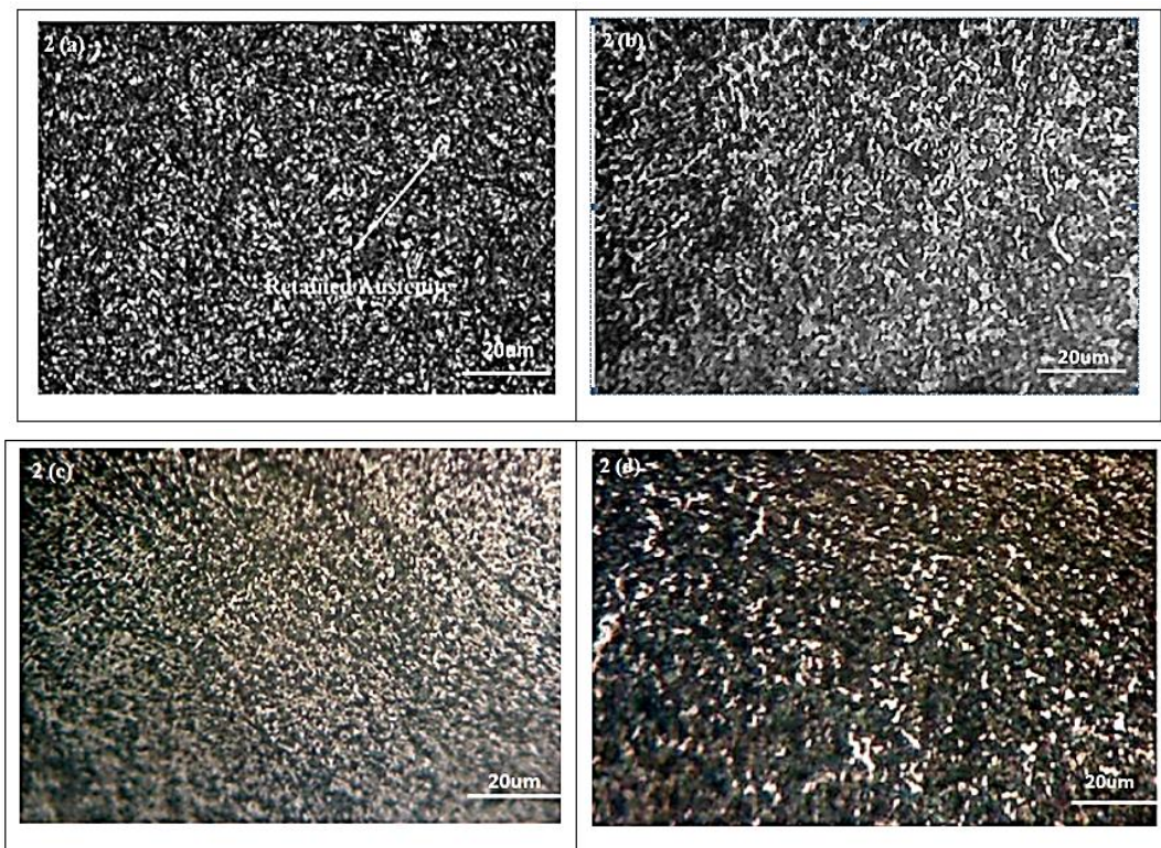
Figure 2. Microstructure of the optimized DCT sample at 20 microns. 2a. The micrograph view of retained austenite on the CHT sample at 20 microns; 2b. The micrograph view of retained austenite the DCT sample at 20 microns; 2c. The micrograph view of flake shaped particles on the CHT sample at 20 microns; 2d. The micrograph view of flake shaped particles on the DCT sample at 20 microns
