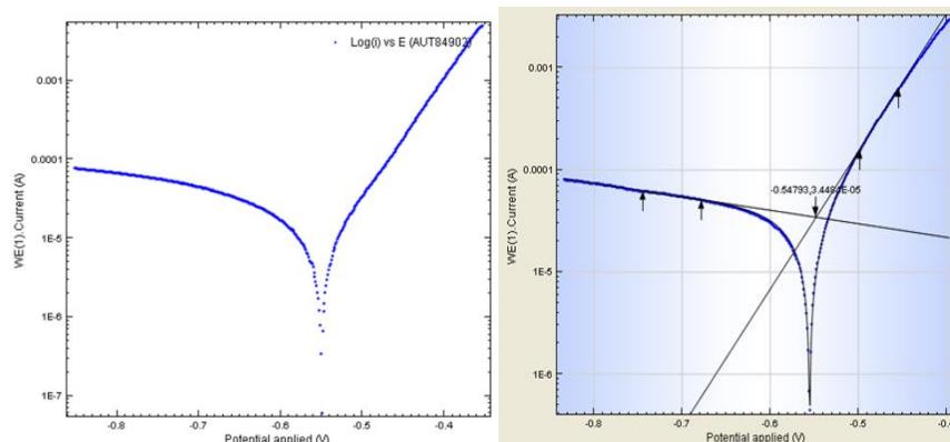
Figure 5. Normal corrosion Tafel plot for CHT samples.
