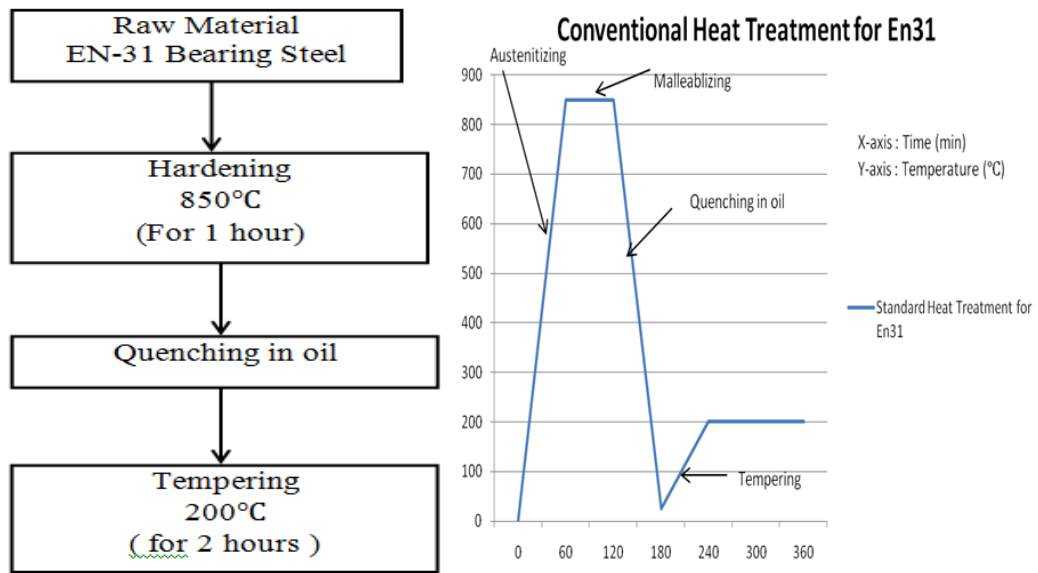
Figure 1. Process chart for conventional heat treatment.
