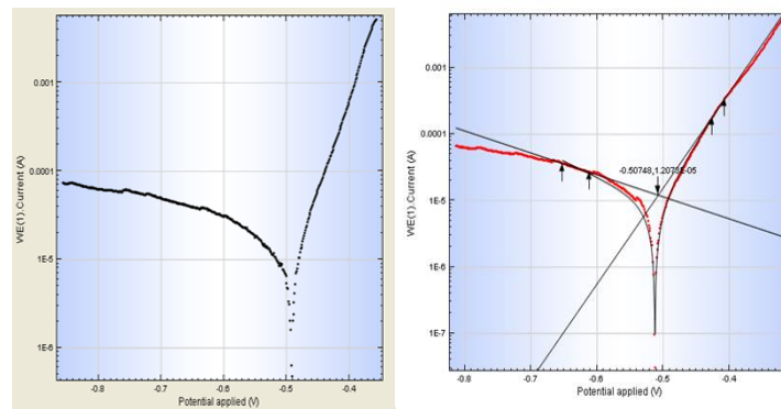
Figure 4. Normal corrosion Tafel plot for DCT samples.
