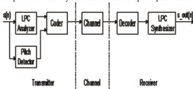
Figure.2: Block Diagram of an LPC Vocoder
