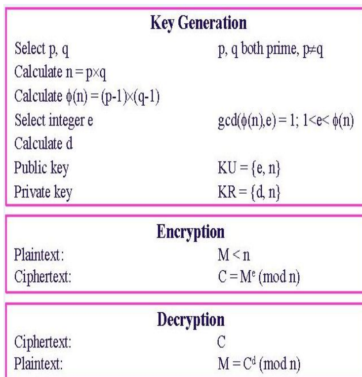
Fig. 2. RSA Algorithm
