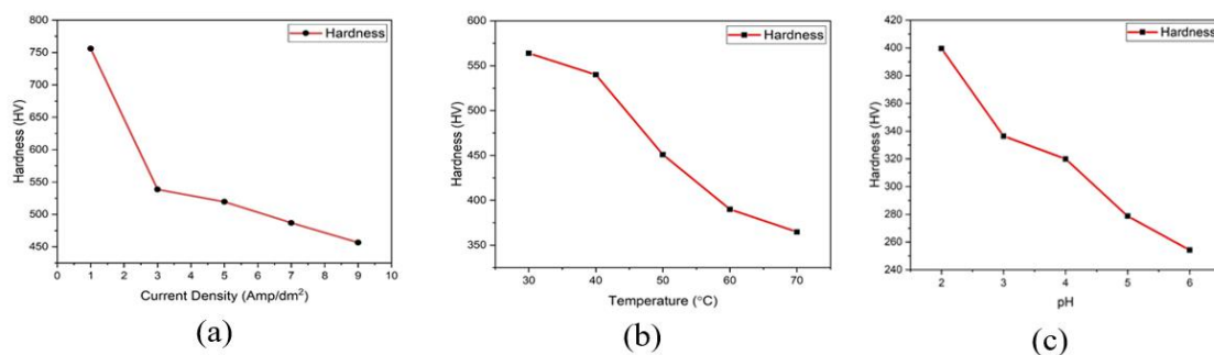
Figure 10. Effect of increasing a) current density; b) processing temperature; c) pH of the electrolyte on microhardness of electroformed nickel.
