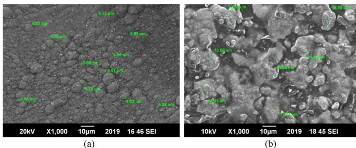
Figure 3. SEM micrographs of the surfaces of electrodeposited nickel developed at two different temperatures a) 30 °C; b) 60 °C.
