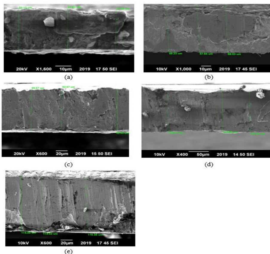
Figure 5. SEM micrographs showing cross section of the nickel-plating samples at various deposition time durations: (a) 1hour (b) 2 hours (c) 3 hours (d) 4 hours (e) 5 hours
