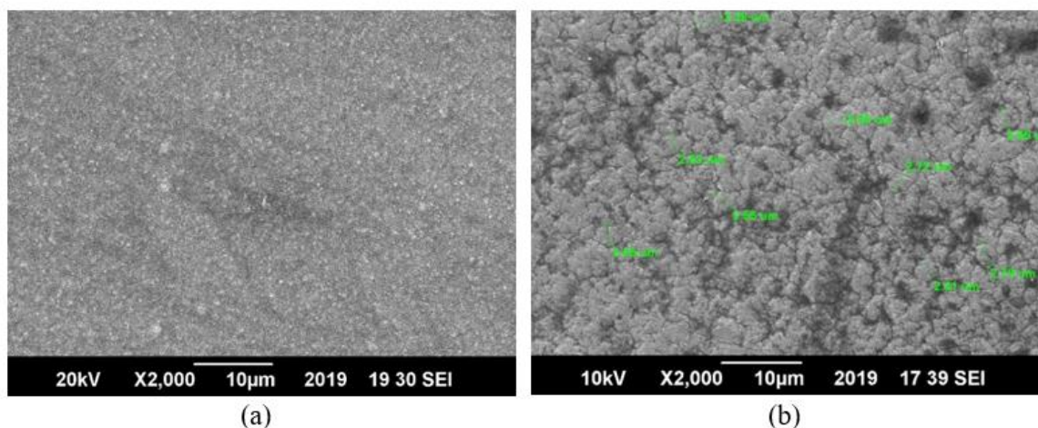
Figure 2. SEM micrographs of the surfaces of electrodeposited nickel developed at two different current densities a) 1 A/dm 2 ; b) 6 A/dm 2 .
