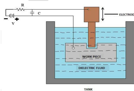
Fig.2. Schematic diagram of Micro-EDM
