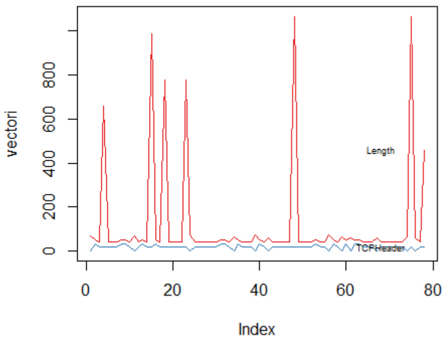
Fig 4. Multivariate between IP payload length and TCP Header Length
