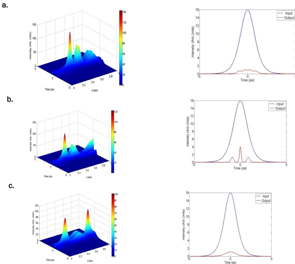
Figure 3. Explain the amplitude of output pulse in three and two dimensions for second order soliton, with different radius air holes. a-d=0.1 μm, b-d=1 μm, c-d=1.8 μm.
