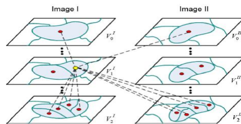
Fig.6. co-multilayer graph model.
