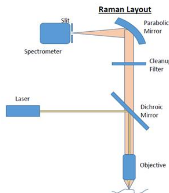
Figure 4B. Raman spectrometers layout.
