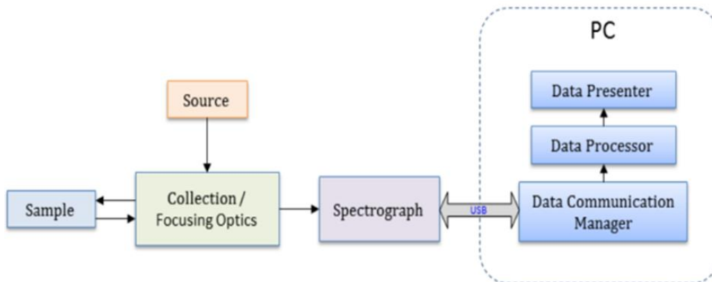
Figure 4A. Raman spectrometers block diagram.
