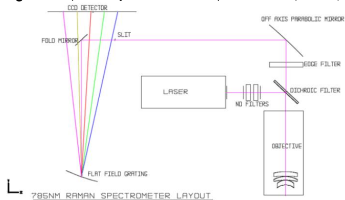
Figure 6. Optical layout of Raman spectrometer (Zemax).
