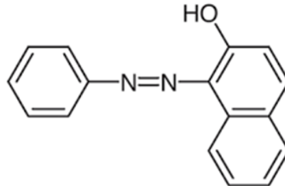
Figure 1. Sudan I molecular structure.
