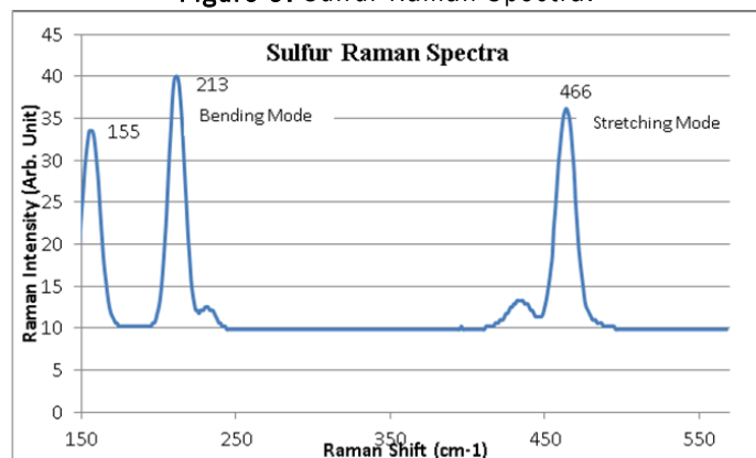
Figure 9. Sulfur Raman Spectra.
