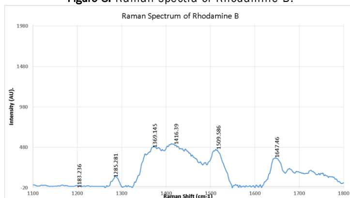
Figure 8. Raman spectra of Rhodamine B.
