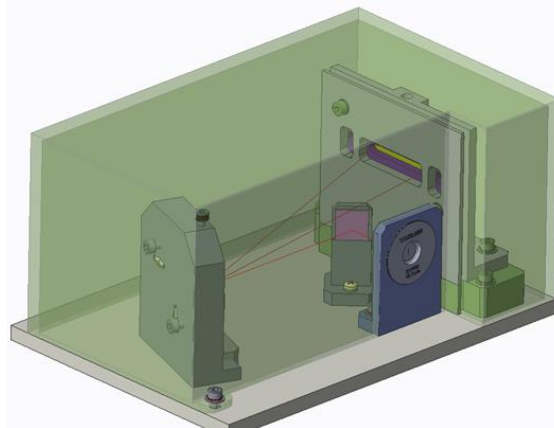
Figure 5. Designed and fabricated Raman spectrograph 3D.
