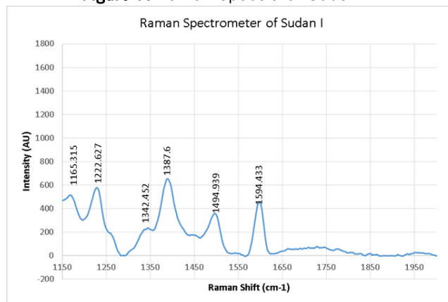
Figure 7. Raman spectra of Sudan I.
