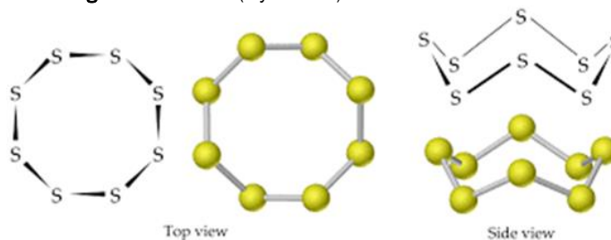
Figure 3. Sulfur (Cyclo-S 8 ) molecular structure.
