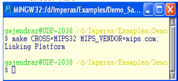
Figure 4: How to Compile the application
