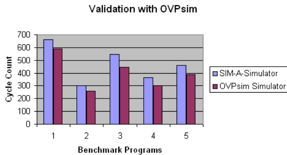
Figure 9: Comparative analysis of SIM-A and OVP Simulator of Cycle Count
