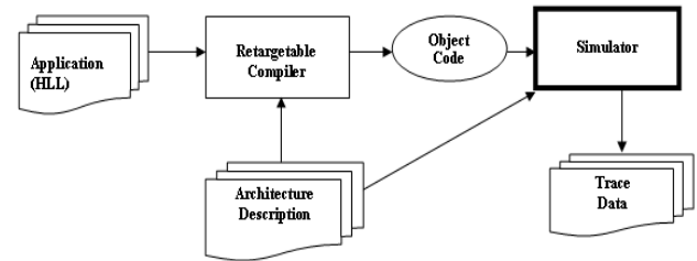
Figure 1: Simulator based code generation
